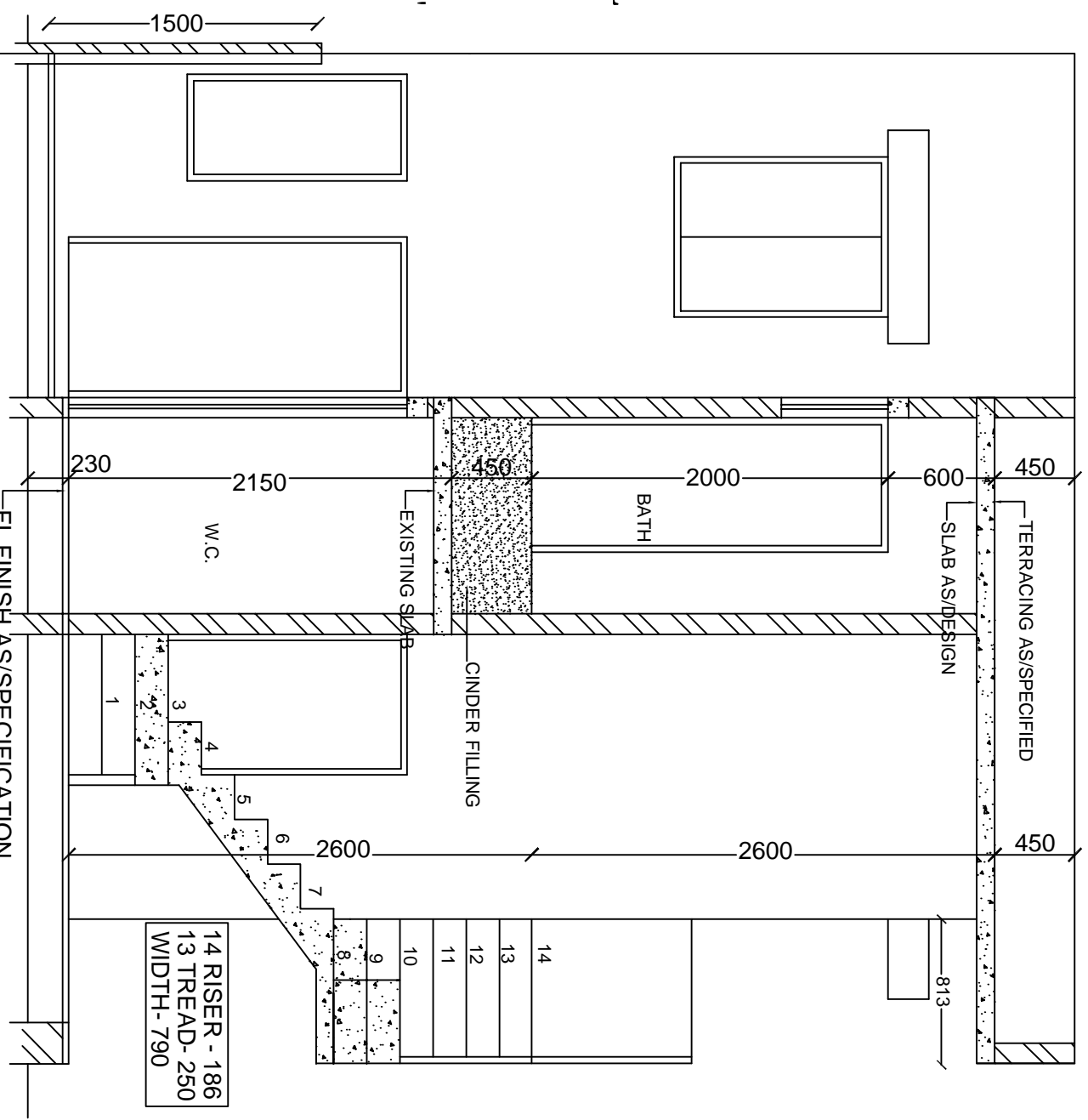
SECTION AT Y-Y' SCALE -1:50
